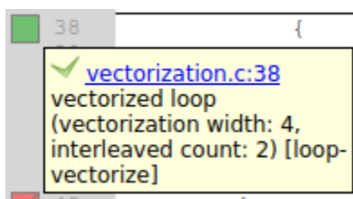
Fig. 11.12: Compiler remark for a successful vectorization attempt after interchanging loop conditions
